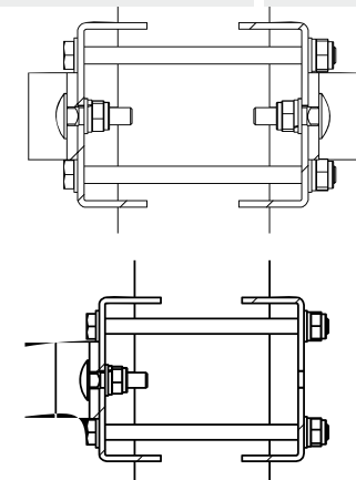
ACCESSORY - GRIP TO PIPE INSTALLATION
