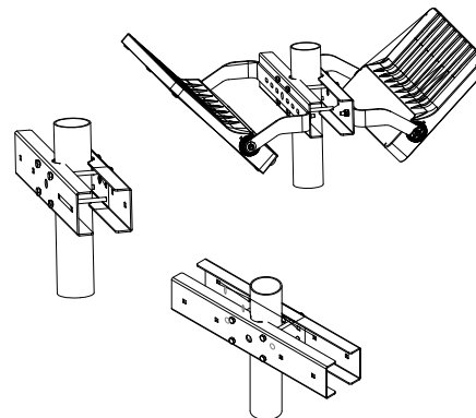
ACCESSORY - APERTURE
